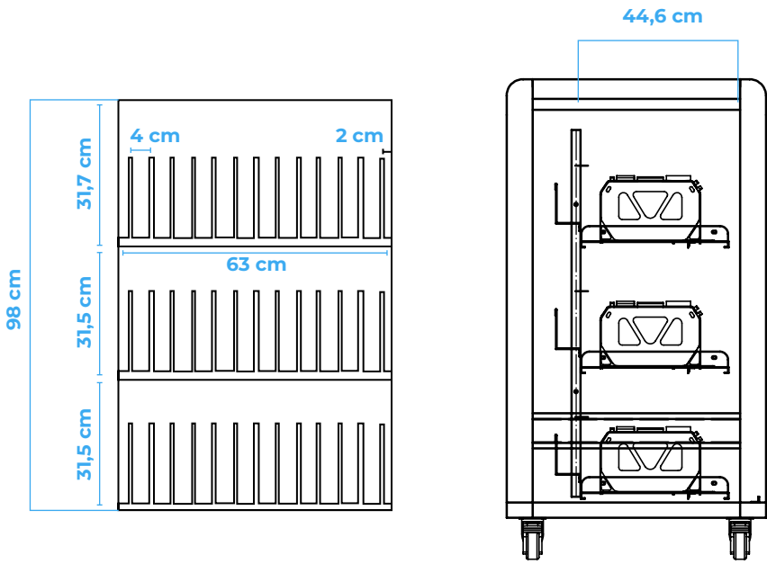
Rear section
