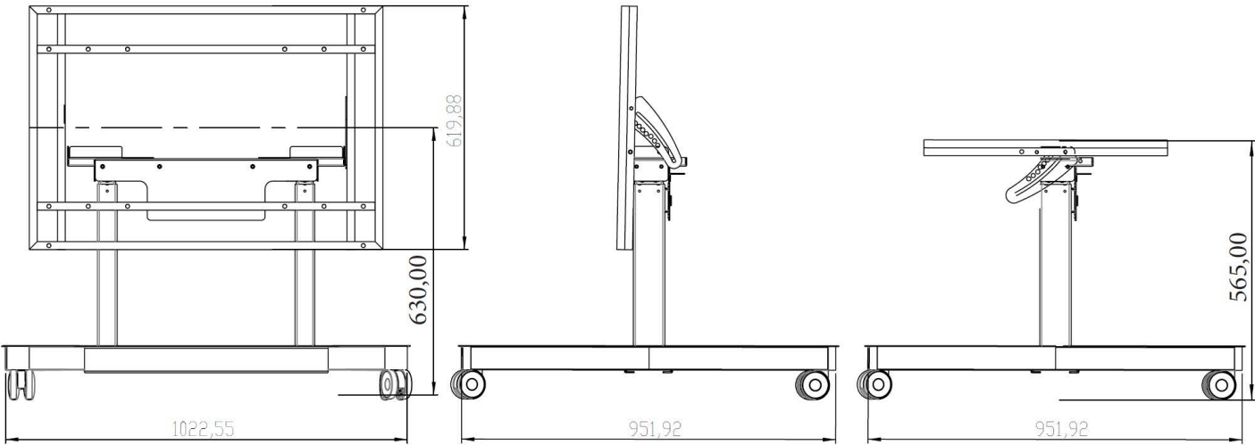
Minimum height / Vertical configuration: 630 mm
