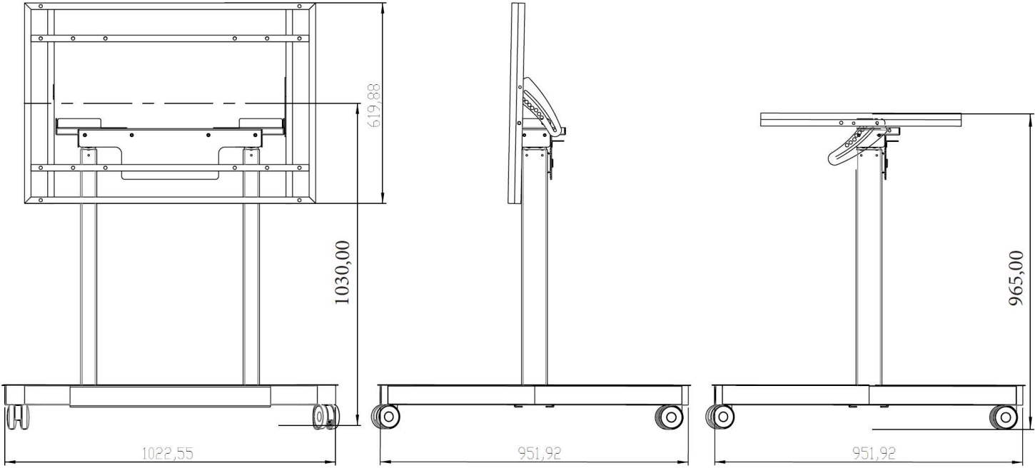
Maximum height / Vertical configuration: 1030 mm
